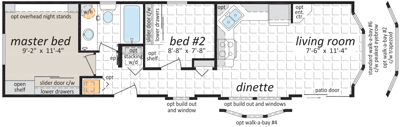
PM-1244-A, 12' x 44'
